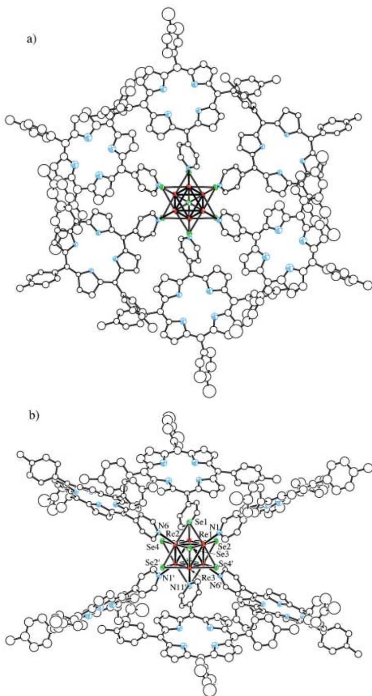
Figure 1. Structure of 3 in 3 \cdot (\text{SbF}_6)_2 \cdot \text{CH}_2\text{Cl}_2 \cdot 1.6 \text{C}_3\text{H}_{12} (ORTEP drawing; thermal ellipsoids at the 30 % probability level). a) Top view, b) side view. Red: rhenium, blue: nitrogen, green: selenium. The crystallographically imposed inversion center is at the center of the \text{Re}_6 octahedron. Selected interatomic distances [Å] and bond angles [°] around the central core: Re–Re: 2.571(2)–2.606(2) (av 2.582); Re–Se: 2.486(4)–2.501(3) (av. 2.483); Re–N: 2.14(2)–2.20(3) (av 2.16); Re–Re–Re (60) : 59.42(6)–60.76(5) (av 60.00); Re–Re–Re (90) : 89.48(7)–90.52(7) (av. 90.00); Re–Se–Re: 62.1(1)–63.4(1) (av 62.7); Se–Re–Se (90) : 89.3(1)–90.6(1) (av 90.0); Se–Re–Se (180) : 176.4(1)–177.1(2) (av 176.7); Se–Re–N: 90.3(7)–93.1(7) (av 91.7).
